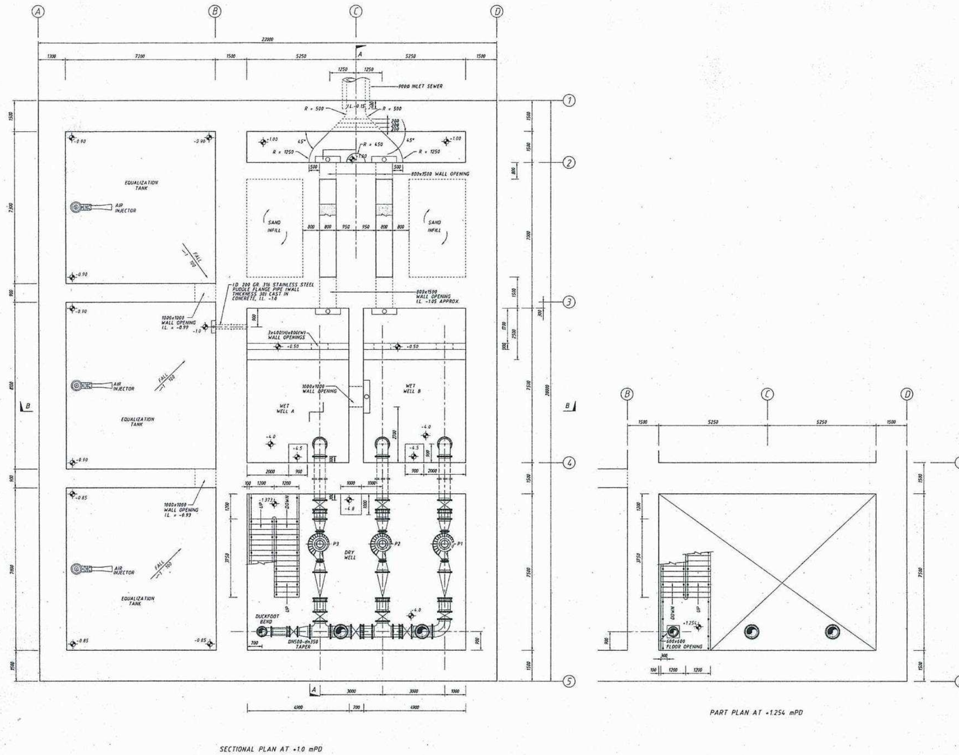
Figure 4: Sewage Pumping Station and Equalization Tanks - Plans
